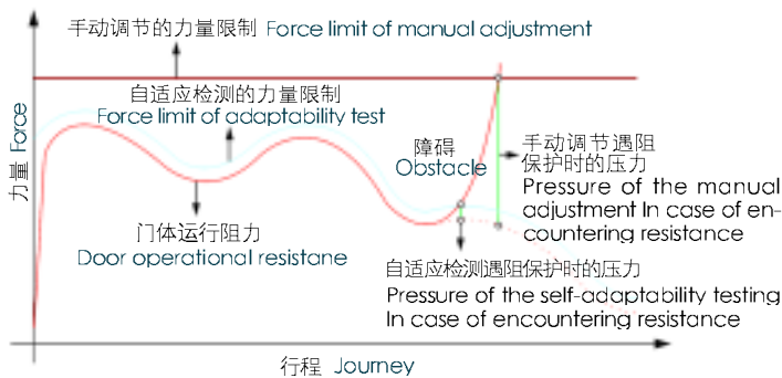
负载力自动跟踪检测曲线图 Curve of the automatic load tracking test
